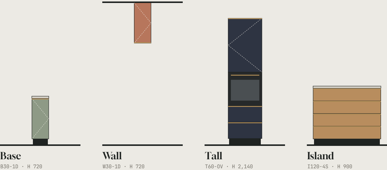
HEIGHTS, DRAWN TO ONE SCALE • SCALE 1:40
